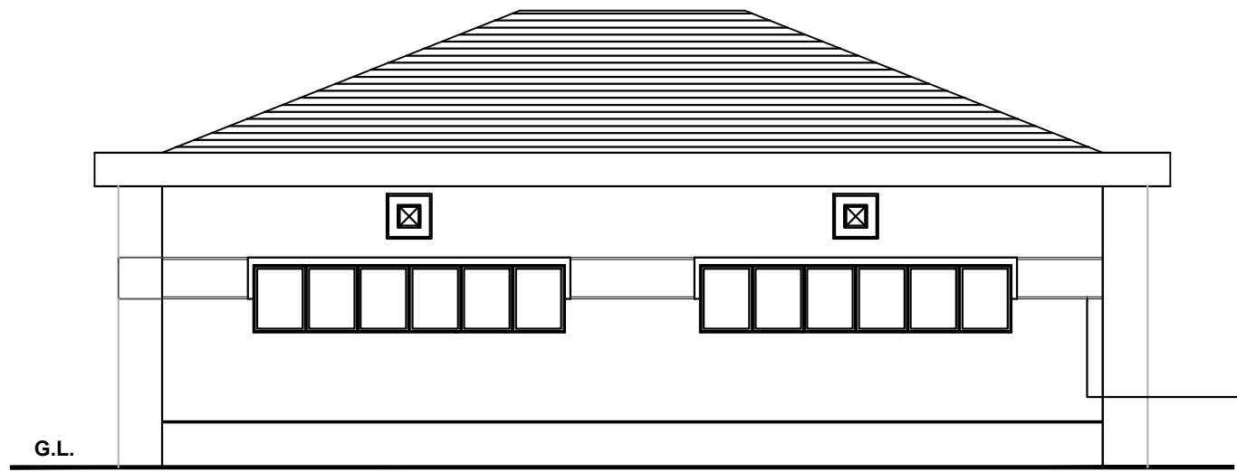
ELEVATION CC
