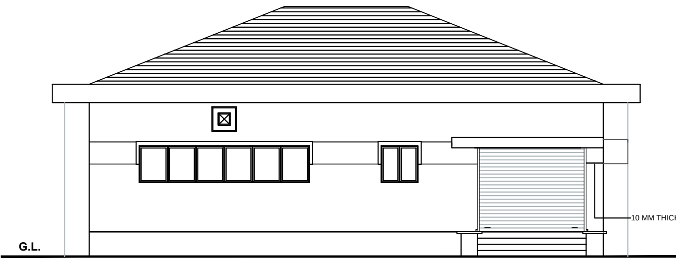
ELEVATION AA
